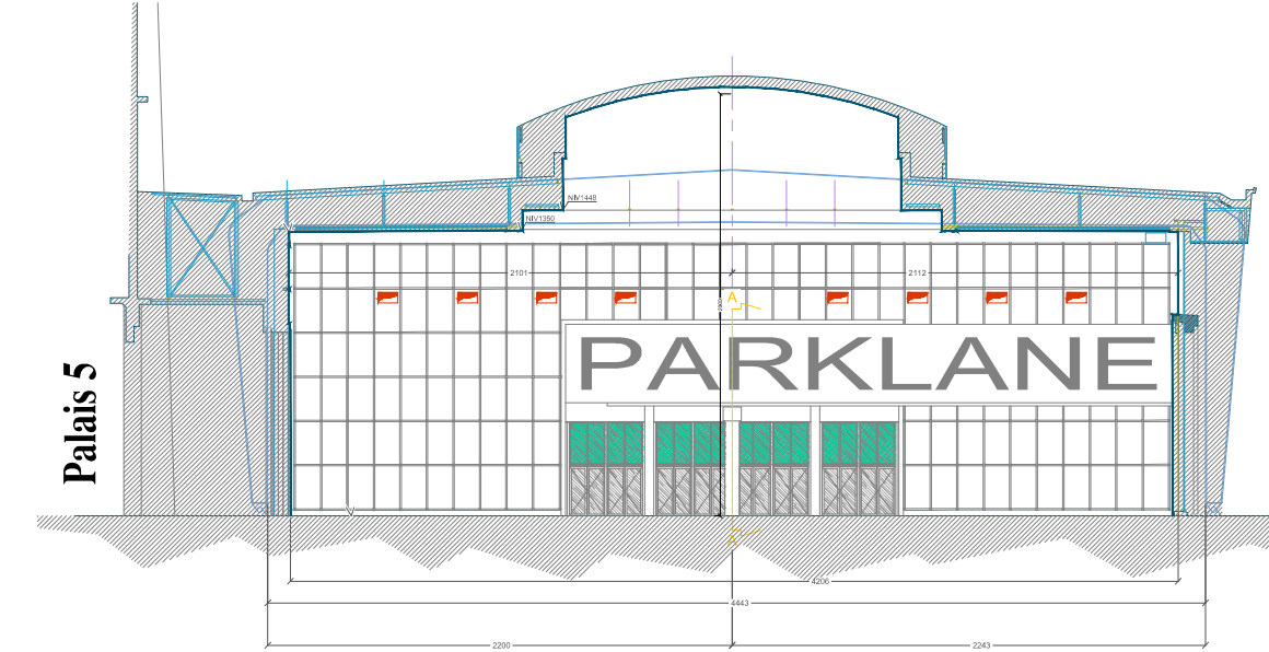
Transversal Section 1/400
