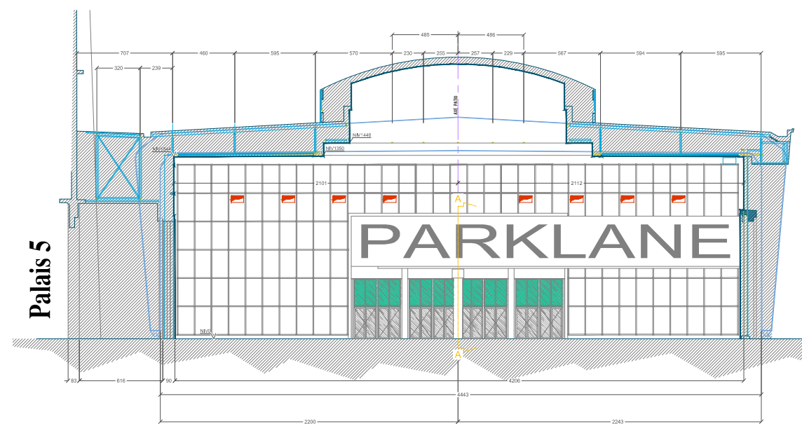
Transversal Section 1/400
