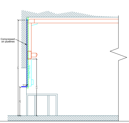
Transversal Section 1/200
